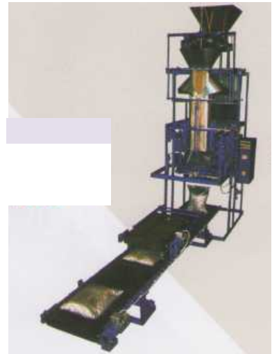
AF-10-V automatic weighing-and-packing machine with a weighing dosing unit
